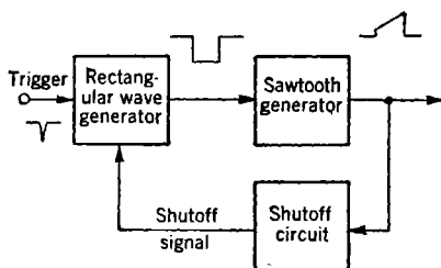
FIG. 4-50.—Alternative combination providing automatic shutoff.
