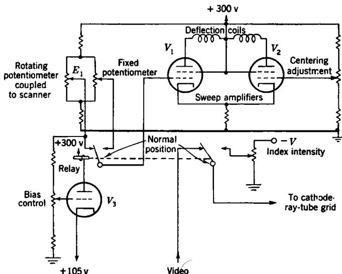
FIG. 6-9.—Substitution index using relay.
