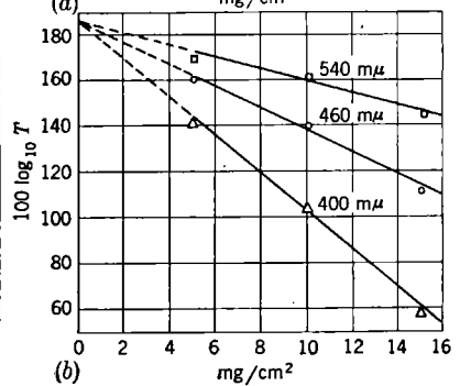
FIG. 18-9.—Plots to determine absorption coefficients at wavelengths shown for two screen materials. T is the transmission in per cent. (a) (93)ZnS:(7)CdS:Cu. (b) (75)ZnS:(25)CdS:Cu.
