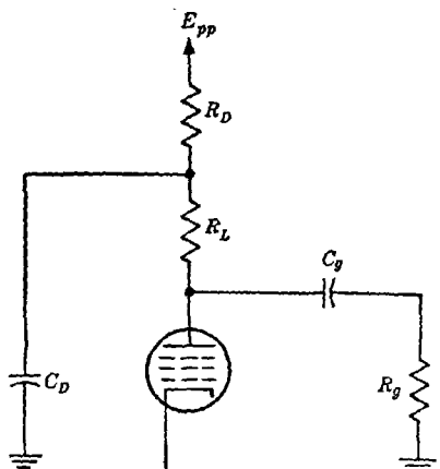
FIG. 4-58.—Plate decoupling used to compensate for droop produced by C_s R_v . R_D \ll R_v ; R_L \ll R_D ; C_D R_D = C_s R_v .
