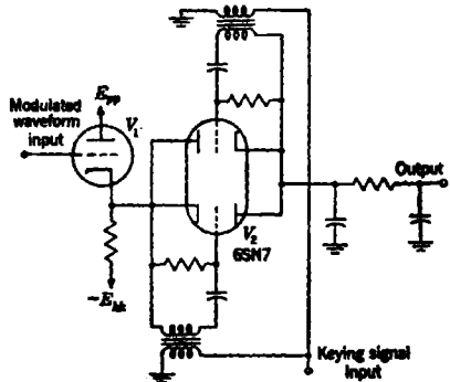
FIG. 5-16.—Keyed detector.
