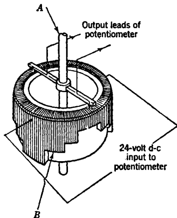
FIG. 5-29.—Potentiometer, type RL-B. See Fig. 11-16 for an application. A , shaft of potentiometer mechanically connected to shaft of scanner; B , resistance winding tapered to correct for load of 200 ohms, so that output voltage is linear with respect to angle of rotation of shaft of potentiometer.
