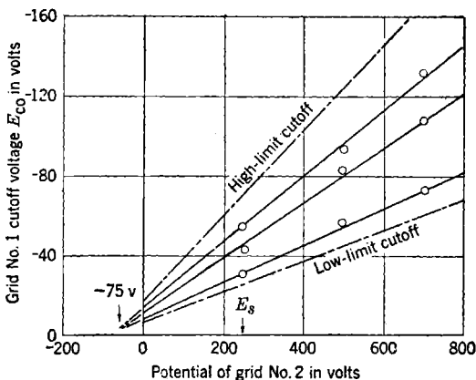
FIG. 2-30.—Variation of cutoff bias with change in second-grid voltage E_{c2} .
