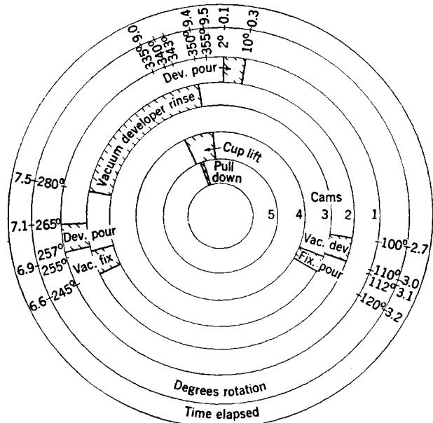
Fig. 16-34.—Cam timing chart; 10-sec cam-shaft cycle.
