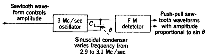
FIG. 5-39.—Modulation of sawtooth waveform by means of sinusoidal condenser.
