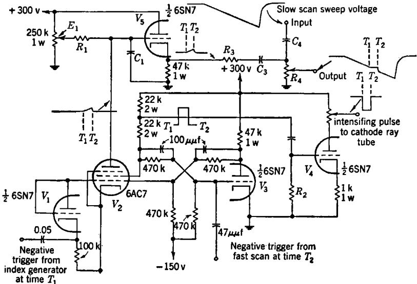
FIG. 6-8.—Sweep-stopping circuit.
